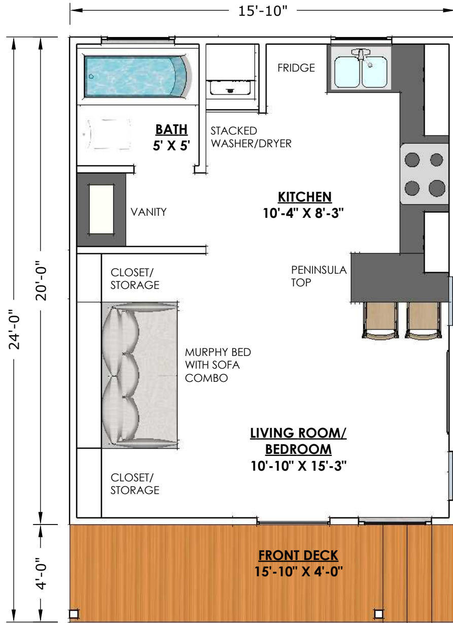
FLOOR PLAN 320 SQ.FT STUDIO
