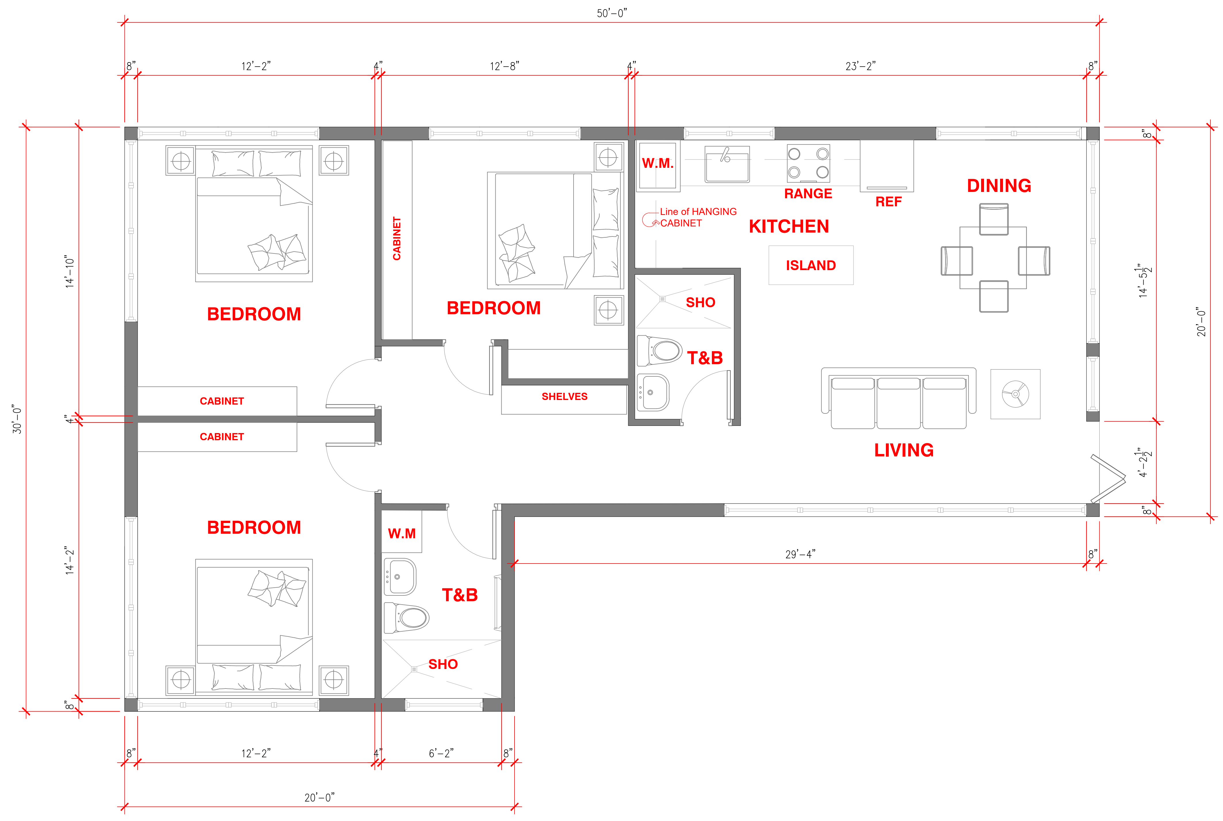
1 A02 GROUND FLOOR PLAN SCALE 3/8" = 1/10"
