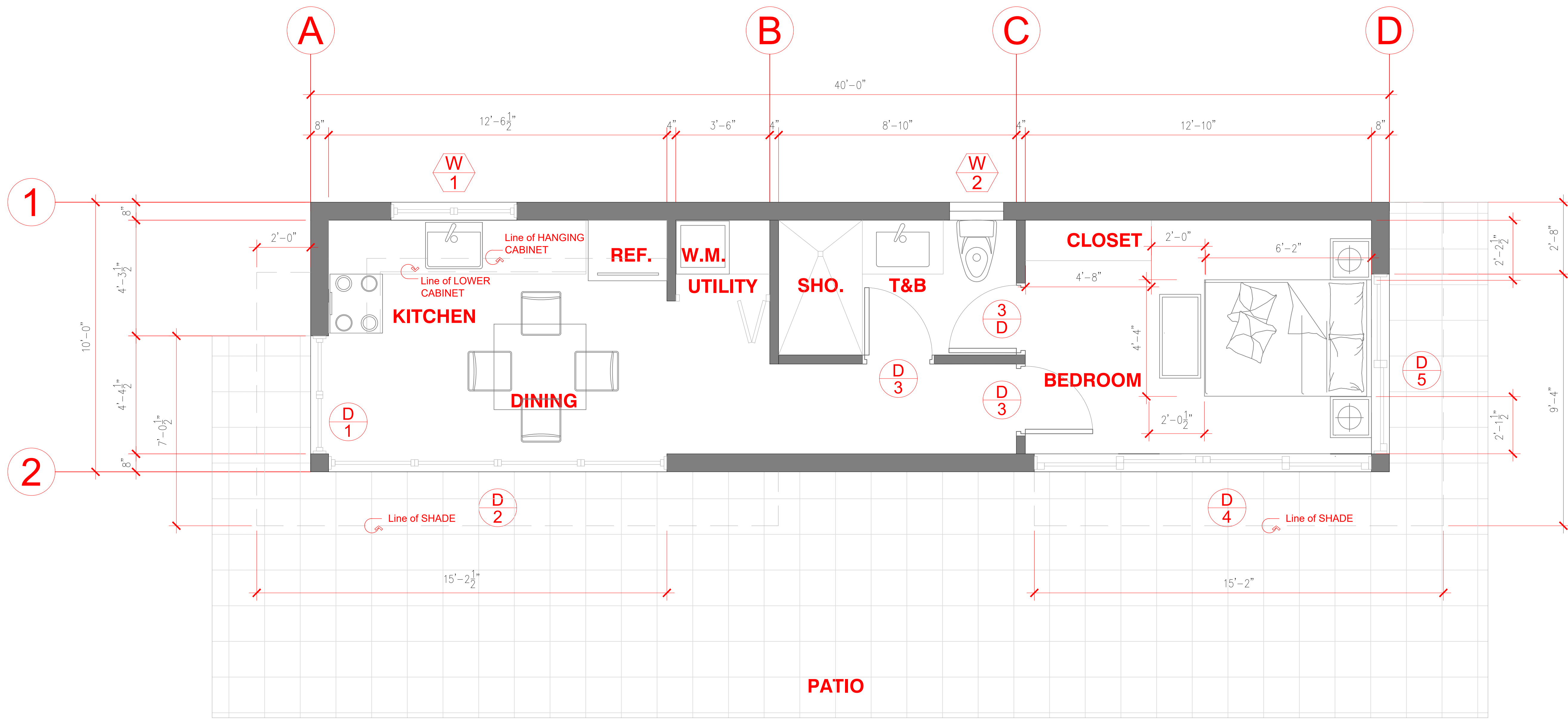
2 GROUND FLOOR PLAN A01 SCALE 3/8" = 1/10"
