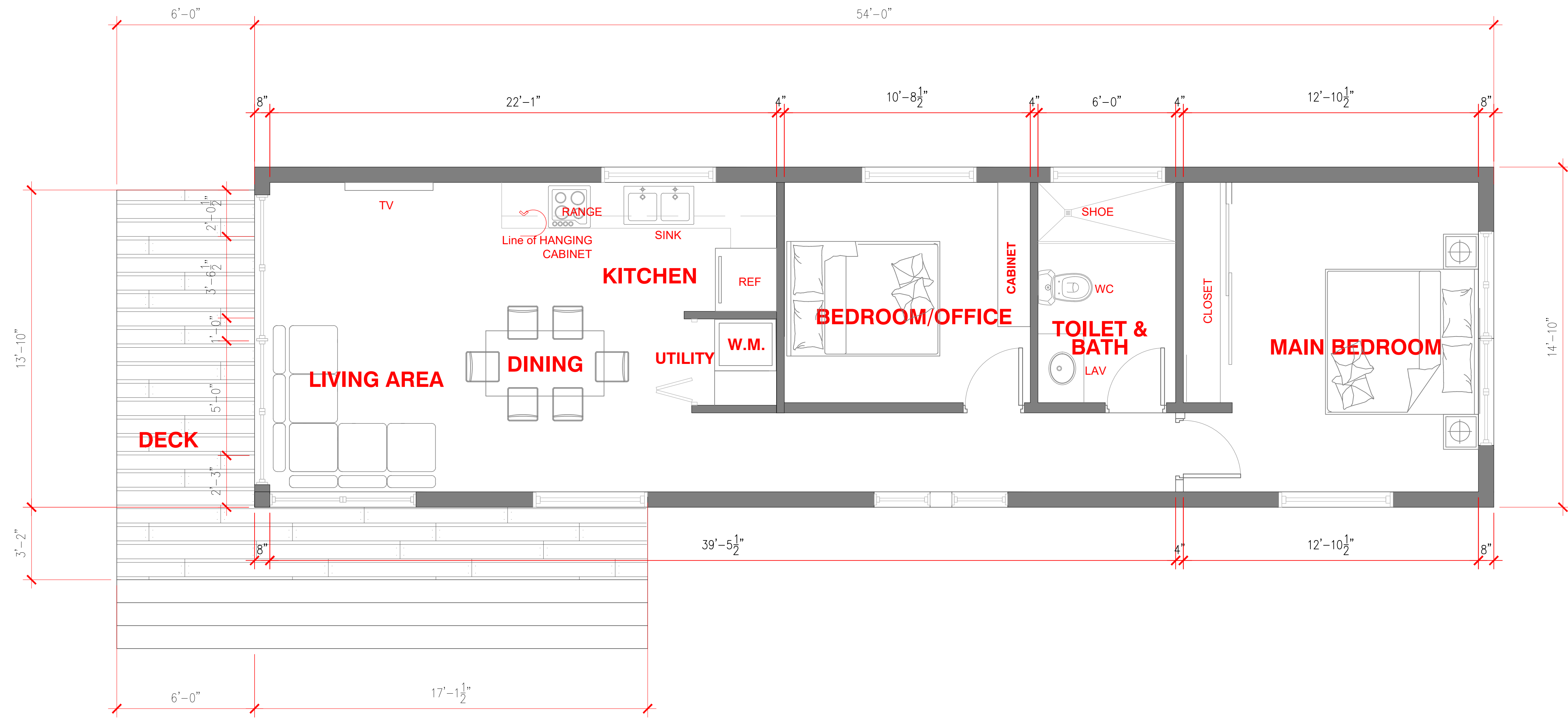
1 A01 GROUND FLOOR PLAN SCALE 3/8" = 1/0"
